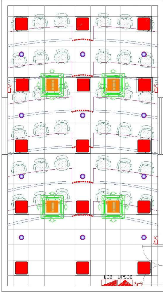
LIGHTING LAYOUT
